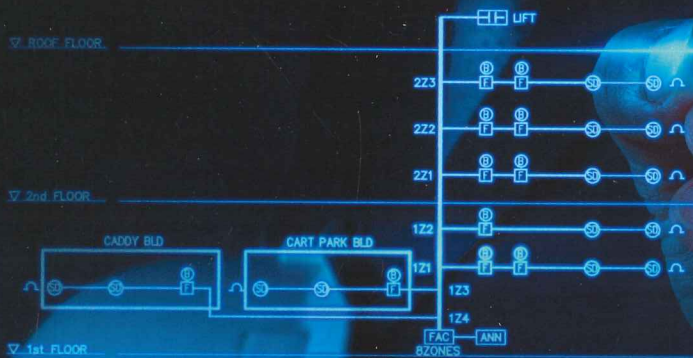
FIRE ALARM RISER DIAGRAM
